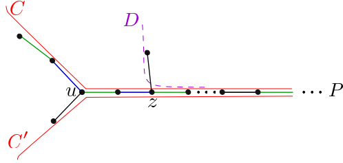
Figure 36: The cycles C, C' and D in the proof of (64).
