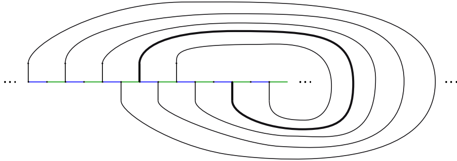
Figure 10: Constructing a consistent embedding in the absence of 2-coloured cycles.
