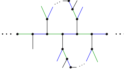
Figure 30: The local situation around a vertex in the case that all edges preserve spin and no 2-coloured cycles exist.
