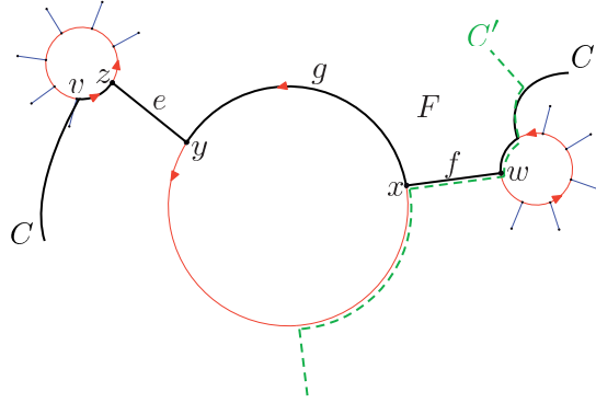
Figure 17: Creating a crossing in Case III.
