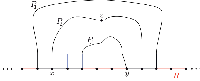
Figure 19: Finding a dividing cycle for the proof of Lemma 9.4.
