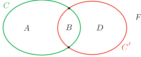
Figure 13: The four regions of \mathbb{R}^2 \setminus (C \cup C') .
