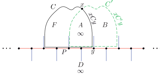
Figure 20: A crossing in the case that p is even.
