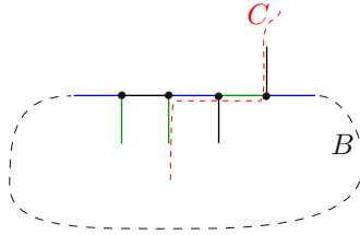
Figure 43: The crossing cycles in the proof of (71).
