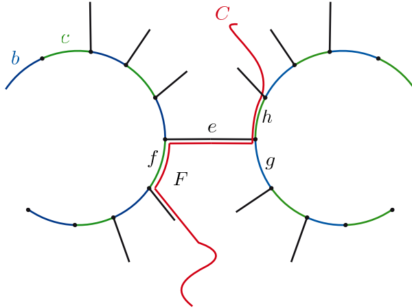
Figure 27: The facial path F in the proof of Lemma 10.2.
