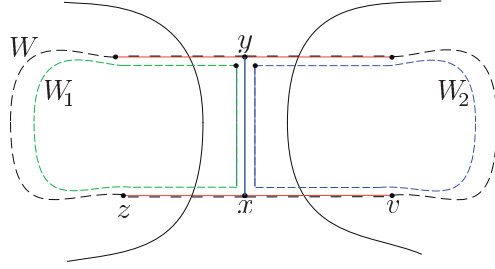
Figure 4: The situation in the proof of (5).
