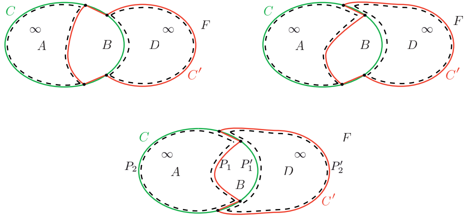
Figure 14: The three ways in which two dividing cycles C, C' can cross. The dashed cycles K, K' are also dividing.
