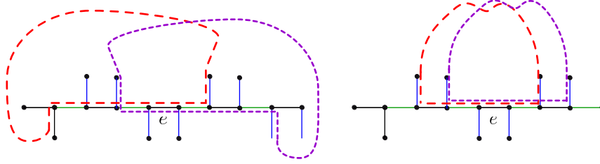
Figure 38: The situation in the proof of (68).
