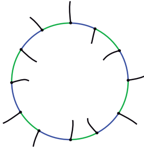
Figure 29: A 2-coloured cycle with mixed spin behaviour.
