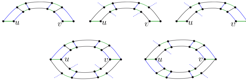
Figure 41: The possible combinations for Z' .
