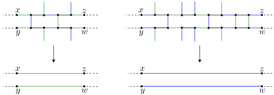
Figure 42: Further reducing operations for the case that d is the dominant colour of C .
