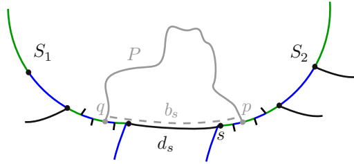
Figure 45: The path P accounting for the 3-connectedness of G .
