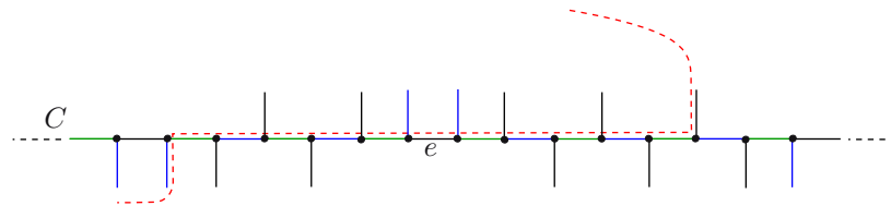
Figure 44: Finding a crossing if two bc-intervals of C have different lengths in the proof of (72).
