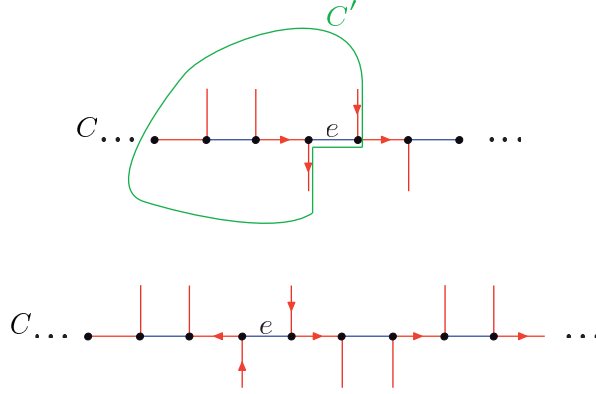
Figure 24: Finding a crossing at an untidy edge e .
