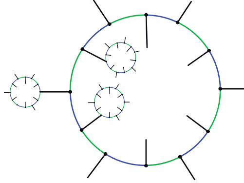
Figure 28: A 2-coloured cycle with spin-preserving edges, and some of its translates.
