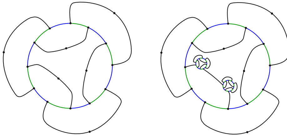
Figure 12: The first step \sigma_0 in the construction of the embedding for the graphs of Case 2 (left) and a possible later step (right).
