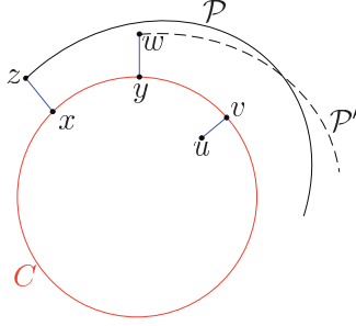
Figure 5: A contradictory situation in the proof of Theorem 6.4.
