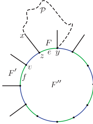
Figure 26: Finding a dividing cycle in the proof of Lemma 10.1.
