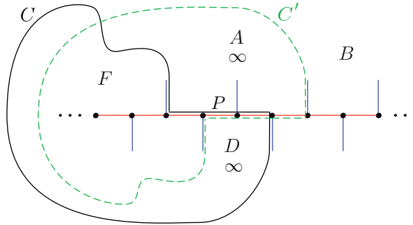
Figure 21: A crossing in the case where p is odd.
