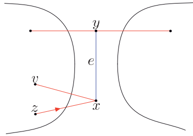
Figure 3: The situation in the proof of (5).
