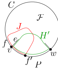
Figure 35: The situation in the proof of (54).
