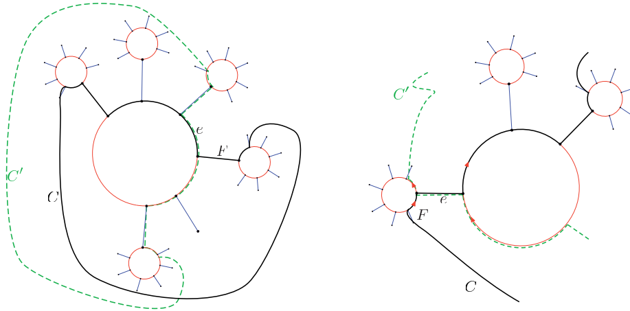
Figure 16: Creating a crossing in Case I (left) and Case II (right).
