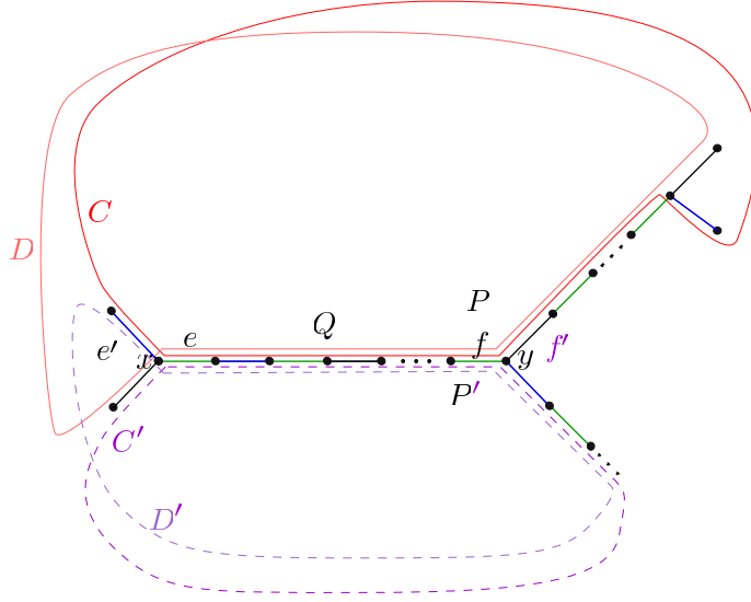
Figure 33: The hypothetical situation when two maximal common subpaths of shortest dividing cycles are not a subpath of each other.
