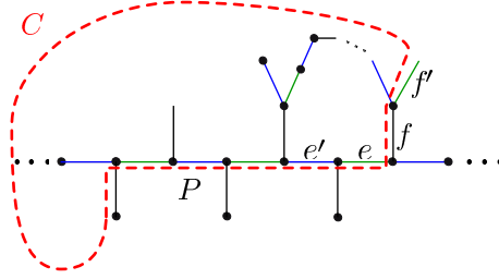
Figure 32: The situation around P in the proof of (41).
