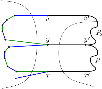
Figure 9: The hypothetical situation when x^{-1}y is not an involution.
