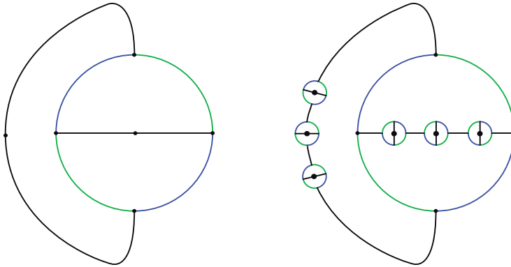
Figure 11: The first step \sigma_0 in the construction of the embedding for the graphs of Case 1 (left) and a possible later step (right). In this example we chose m = 4 , i.e. our graph is \text{Cay} \langle b, c, d \mid b^2, c^2, d^2, bc bc, (bcd)^4 \rangle .
