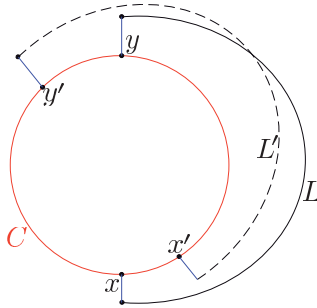
Figure 6: A contradictory situation in the proof of Theorem 6.4.
