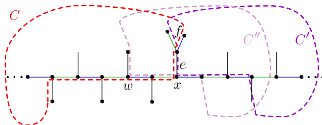
Figure 37: The construction of D in the proof of Proposition 10.16.
