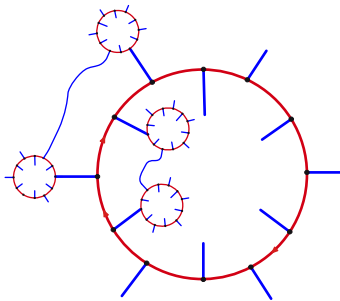
Figure 18: An a -cycle and some of its translates. Every a -edge reverses spin.
