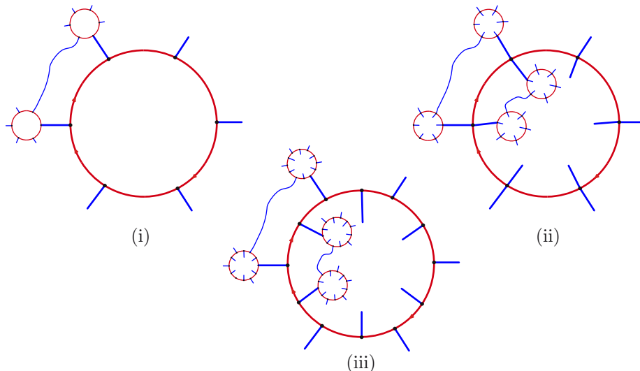
Figure 1: A twist-amalgamation.
