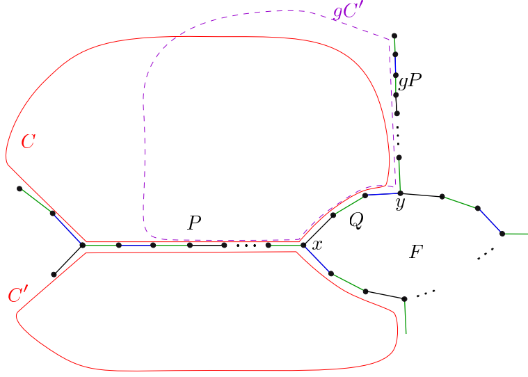
Figure 34: The situation arising in the proof of (49).
