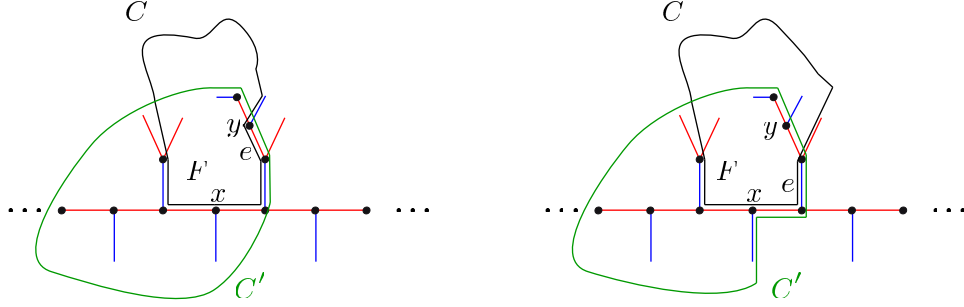
Figure 22: Proof that a facial subpath of length four forces a crossing.
