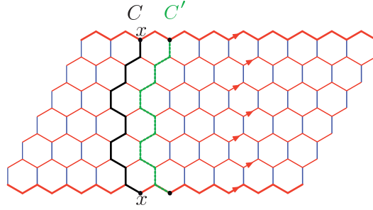
Figure 25: The case when every face is a hexagon and b reverses spin, and a shortest dividing cycle C . The top and bottom rays coincide, and so do the two vertices marked x .
