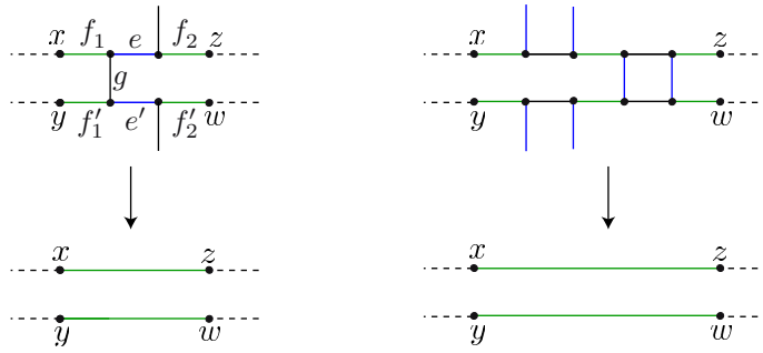
Figure 39: Two operations that simplify Z without changing its curvature.
